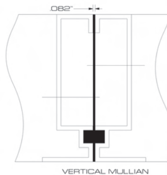
VERTICAL MULLIAN
