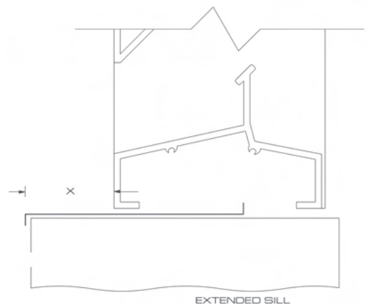
EXTENDED SILL
