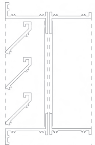
SLEEVE
